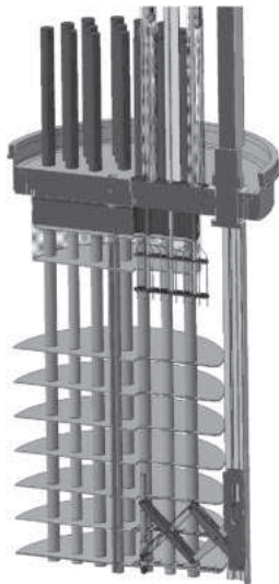
Fig. 5 Slitted ACS
