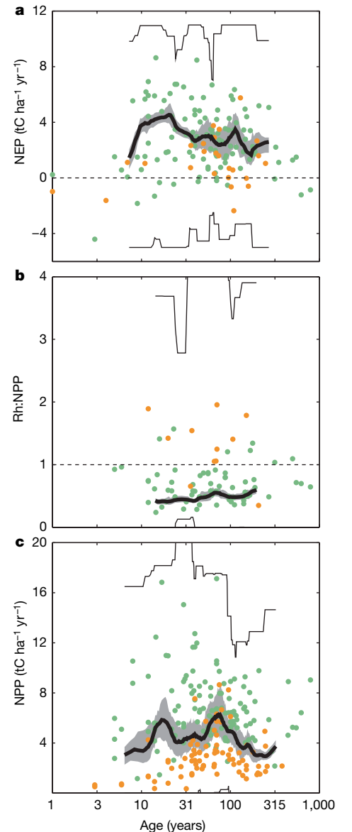
Figure 1 — Changes in carbon fluxes as a function of age. a, Observed NEP versus age; positive values indicate carbon sinks and negative values indicate carbon sources. b, Observed ratio of heterotrophic respiration (Rh) to NPP versus age; Rh:NPP < 1 indicates a carbon sink. c, Observed NPP versus age. It appears that temperate and boreal forests both show a pattern of declining NPP. Most probably, the late-successional increase in NPP is caused by the combination of data from different climate regions or the combination of disturbance regimes (Supplementary Fig. 2a, b). In each panel, the green dots show observations of temperate forests, the orange dots show observations of boreal forests, the thick black line shows the weighted mean within a moving window of 15 observations, the grey area around this line shows the 95% confidence interval of the weighted mean and the thin black lines delineate the 95% confidence interval (where visible) of the individual flux observations.
