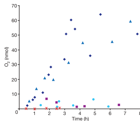
Figure 4 | Oxygen production from nitrite in Methyloirabilis oxyfera . Whole cells of enrichment culture 'Ooij' were incubated in buffer containing nitrite and 25\% ^{18}\text{O} -labelled water, leading to 90\% O exchange within 30\text{ min} . Total oxygen production from this indirectly labelled \text{N}^{18}\text{O}_2^- was inferred from the measured concentration of ^{16,18}\text{O}_2 and ^{18,18}\text{O}_2 in the helium headspace with the following additions: propylene (dark blue diamonds), propylene and acetylene (blue triangles), methane (purple squares) and oxygen (light blue circles). Anaerobic control incubations of Methylosinus acidophilus (red asterisks) with ^{18}\text{O} -labelled nitrite did not produce measurable amounts of oxygen. Cells were concentrated to obtain similar maximum rates of propylene oxidation activity; 1.15\text{ nmol min}^{-1} (with \text{NO}_2^- , 1.22\text{ mg} of protein) for ' M. oxyfera ', and 1.68\text{ nmol min}^{-1} (with \text{O}_2 , 0.046\text{ mg} of protein) for M. acidophilus .
