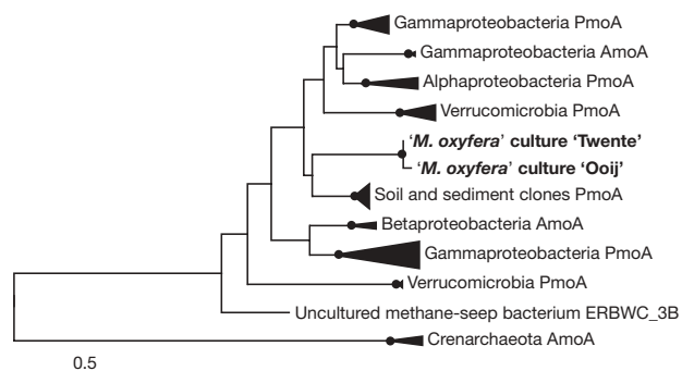
Figure 2 | Phylogeny of ' Methyloirabilis oxyfera ' pmoA protein sequences. Neighbour-joining tree showing the position of enrichment cultures 'Twente' and 'Ooi' (in bold) relative to other pmoA and amoA sequences. The distance tree was computed with the Dayhoff matrix-based method, and bootstrapping of 100 replicates was performed within the neighbour-joining, minimum-evolution, maximum-parsimony and maximum-likelihood evolutionary methods. Bootstrapping results are summarized on the tree, with filled circles representing branch points at which all four methods give greater than 70% support. The scale bar represents 50 amino-acid changes per 100 amino acids. See also Supplementary Fig. 3 for more detailed tree and bootstrap values.
