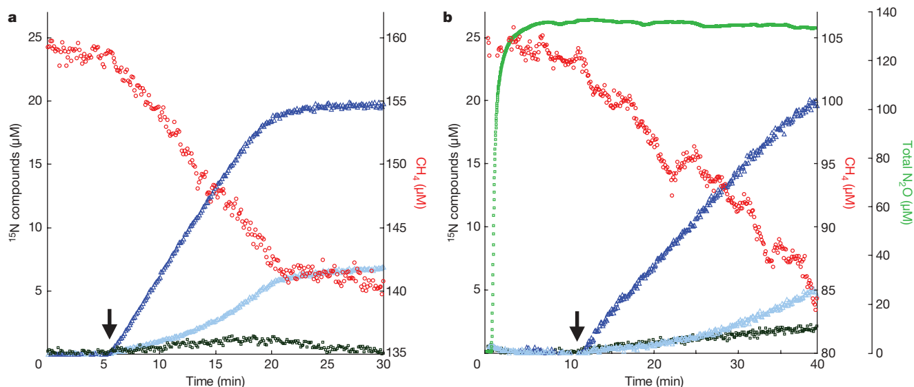
Figure 3 | Coupling of methane oxidation and nitrite reduction in enrichment cultures of Methyloirabilis oxyfera . Methane is oxidized only after addition of ^{15}\text{N} -labelled nitrite ( 50\text{ }\mu\text{M} , arrow), which is converted to ^{15}\text{N} -labelled dinitrogen gas in the presence of about 2,000\text{ }\mu\text{M} ^{14}\text{N} -nitrate (a) or 2,000\text{ }\mu\text{M} ^{14}\text{N} -nitrate and 135\text{ }\mu\text{M} ^{14}\text{N} - \text{N}_2\text{O} (b). Experiments were
