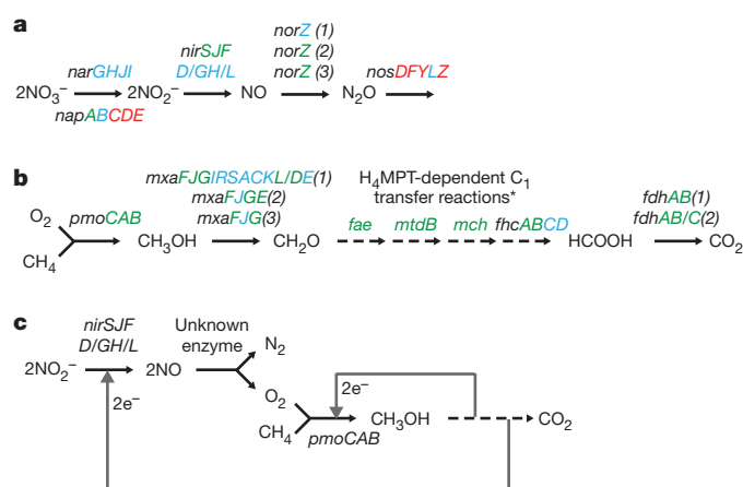
Figure 1 | Significant pathways of Methyloiridis oxyfera . Canonical pathways of denitrification (a), aerobic methane oxidation (b) and proposed pathway of methane oxidation with nitrite (c). narGHJI , nitrate reductase; napABCDE , periplasmic nitrate reductase; nirSJFD/GH/L , nitrite reductase; norZ , nitric oxide reductase; nosDFYLZ , nitrous oxide reductase; pmoCAB , particulate methane monooxygenase; mxafJGIRSAKCL/DE , methanol dehydrogenase; fae , formaldehyde-activating enzyme; mtdB , methylene-tetrahydrodihydropterin (H 4 MPT)-dependent C 1 transfer reactions; mch , methenyl-H 4 MPT cyclohydrolase; fhcABCD , formyltransferase/hydrolase; fdhABC , formate dehydrogenase. Genes in red are absent from the genome, those in blue are present in the genome and those genes in green are present in both the proteome and the genome. Asterisk, H 4 MPT-dependent reactions involve the intermediates methylene-H 4 MPT, methenyl-H 4 MPT and formyl-H 4 MPT.
