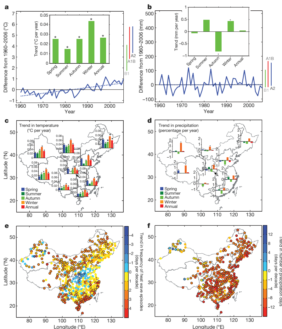
Box 1 Figure · Observed trends and future projections of climate in China. a , Observed mean annual temperature variations between 1960 and 2006 across the country, expressed as deviation from the mean during that period (blue line). The blue dotted line is a fit to the data: y = 0.0263x - 52.13 ( R^2 = 0.54 , P = 0.001 ). The inset shows trends in seasonal temperature (°C per year) during the period 1960–2006. The data come from the climate records of 412 meteorological stations. The three coloured bars on the right-hand side show the projected temperature range by 2100 for the three IPCC marker scenarios A1B, A2 and B1. Model output comes from ref. 1 and uses an ensemble of 24 models. b , As for a but for precipitation variations, but the data come from climate records at 355 meteorological stations where all daily precipitation data are available during the period of 1960–2006. The blue dotted line is a fit to the data:
