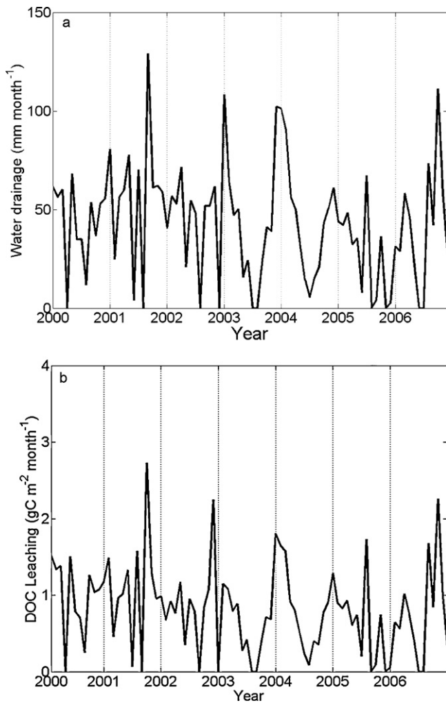
Fig. 3. Monthly water drainage ( \text{mm month}^{-1} ) averaged over the full study period (2000–2006) (panel a). Monthly DOC-leaching ( \text{gC m}^{-2} \text{ month}^{-1} ) for the full study period (2000–2006), as calculated the product of monthly DOC concentration measured at Cg horizon and water drainage (panel b).
