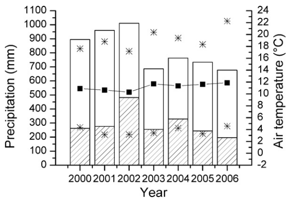
Fig. 1. Meteorological conditions at 'De Inslag', Brasschaat, Belgium during the study period (2000–2006). The bar graph shows the annual precipitation (left ordinate) which is divided into growing season (open bars) and dormant season (dashed bars). Filled squares show mean annual air temperature (right ordinate) and the upper and lower asterisk show highest and lowest mean monthly temperature for that specific year.
