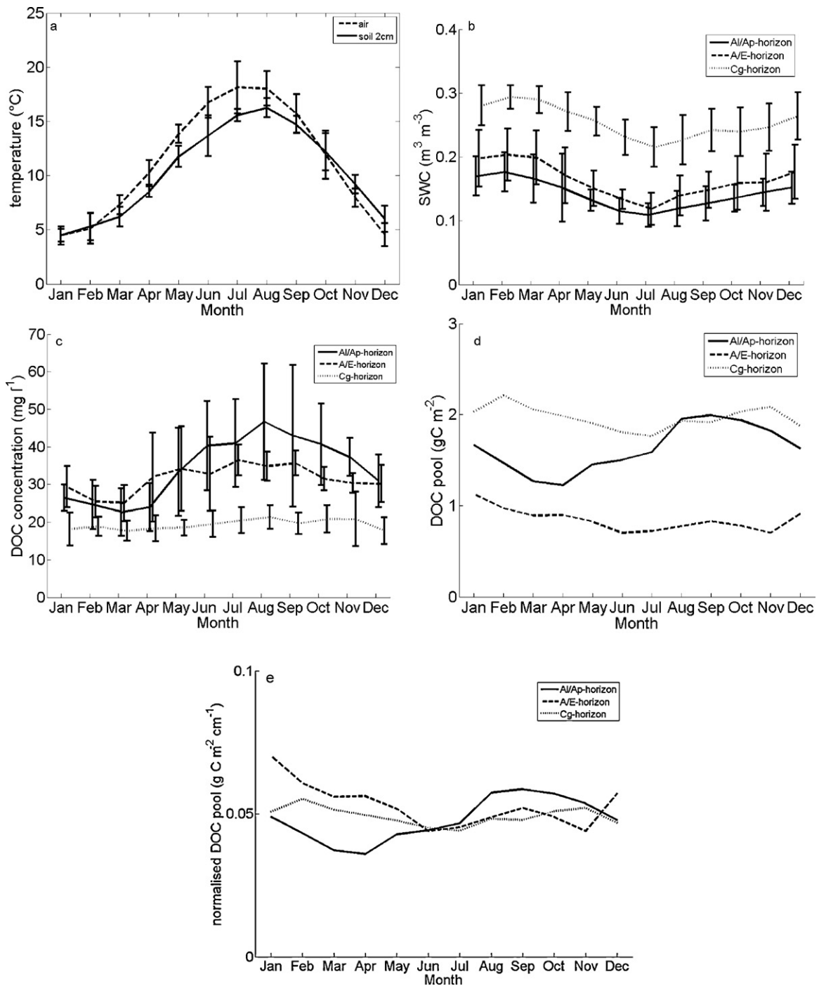
Fig. 2. Seasonal patterns of air temperature ( ^{\circ}C ) and soil temperature at 2 cm below soil surface ( ^{\circ}C ) (panel a); SWC ( m^3 m^{-3} ) measured in the different soil horizons Al/Ap, A/E and Cg (panel b); DOC concentrations ( mg l^{-1} ) in the different soil horizons Al/Ap, A/E and Cg (panel c) and DOC pool ( gC m^{-2} ), calculated as the product of DOC concentration and SWC at the three soil horizons (panel d). A normalised pool ( gC m^{-2} cm^{-1} ) for each horizon was calculated by dividing the pools by their depth (panel e). In each panel, data are mean monthly averaged over the 7-year period.
