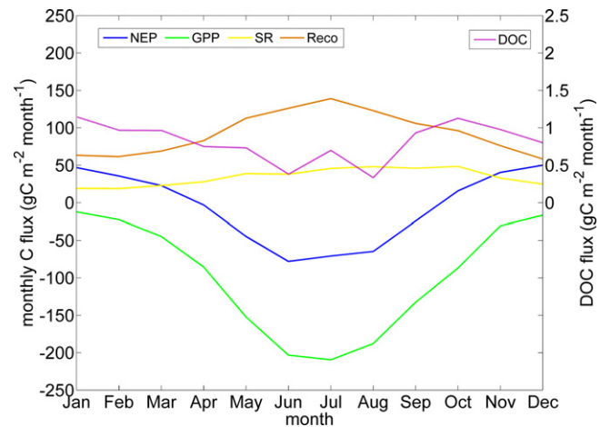
Fig. 5. Mean seasonal pattern over the entire study period for GPP, Reco, NEP and SR ( \text{in gC m}^{-2} \text{ month}^{-1} ) on the left ordinate and DOC fluxes on the right ordinate ( \text{gC m}^{-2} \text{ month}^{-1} ). Scale differs in both Y-axis.
