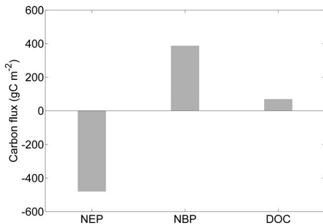
Fig. 4. Mean NEP, NBP and DOC over a 6-year period (2000–2006, omitting 2003 due to lack of NEP data), all expressed in ( \text{gC m}^{-2} ).
