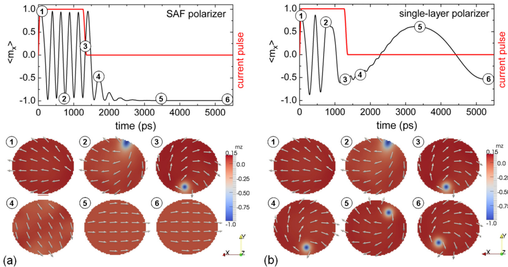
FIG. 3. (Color online) Simulations for a current density J_{\text{app}}=2.5 \times 10^{11} A/m 2 and pulse length \Delta t=1210 ps with a SAF polarizer (a) and a single-layer polarizer (b). The color scale represents the out-of-plane component of the magnetization. In (b), when the current is off, the vortex describes a spiral around the FL center. The system is at static equilibrium when the vortex reaches the center.
