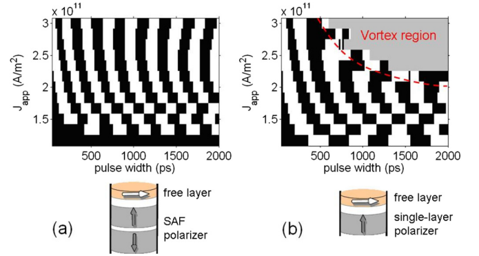
FIG. 2. (Color online) Switching probability as a function of pulse width and current density for a SAF-polarizer (a) and a single-layer polarizer (b). Black: P_s=0 (the final state is the same as the initial state). White: P_s=1 (the final state is opposite to the initial state). Gray: the final state is a vortex. The current density ranges from 1.17 \times 10^{11} – 3 \times 10^{11} A/m 2 by 0.17 \times 10^{11} A/m 2 step. The pulse width ranges from 50 to 1990 ps by 20 ps step.
