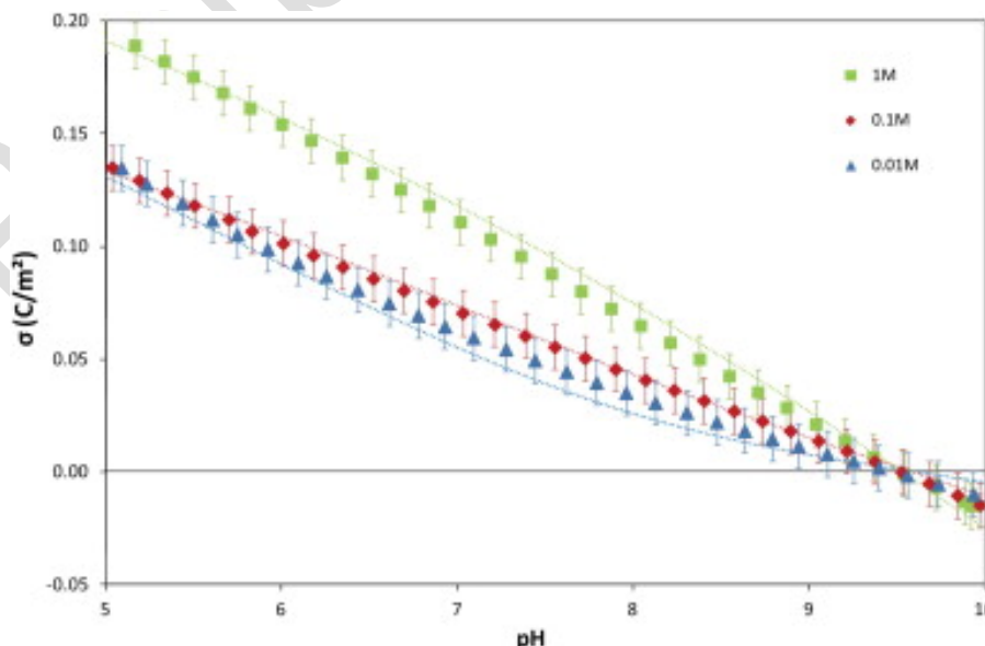
Figure 1. Surface charge of \alpha\text{-Al}_2\text{O}_3 at different pH and ionic strengths. The dotted lines are the results of modelling.
