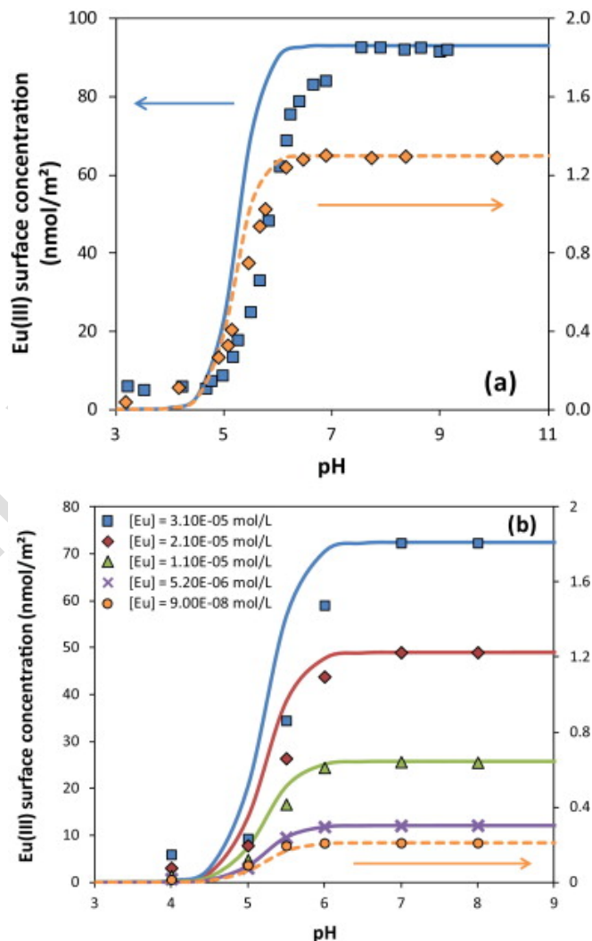
Fig. 3. Eu(III) surface concentration on (a) 4.4 g/L hydrous alumina ( 105 \text{ m}^2/\text{g} ), for I = 0.1 \text{ M KNO}_3 and [\text{Eu(III)}] = 4.3 \cdot 10^{-5} \text{ mol/L} (squares) and 0.1 \text{ M NaClO}_4 and [\text{Eu(III)}] = 6.0 \cdot 10^{-7} \text{ mol/L} (diamonds) [21]; (b) 3.6 g/L \gamma\text{-Al}_2\text{O}_3 ( 119 \text{ m}^2/\text{g} ) for I = 0.1 \text{ M NaClO}_4 and various Eu(III) concentrations [22]. Symbols are the data from literature, and lines are the results of our modelling.
