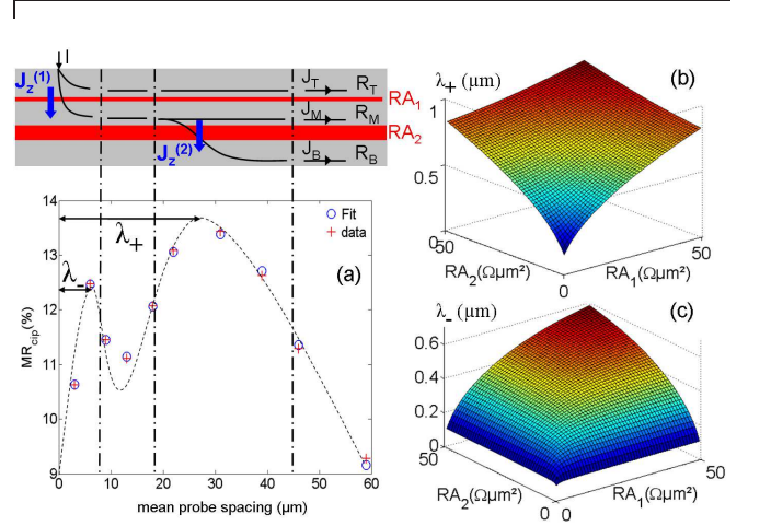
FIG. 3. (a) Comparison of Capres data with our model using RA_1 = 700\Omega\cdot\mu m^2 , RA_2 = 12.6k\Omega\cdot\mu m^2 , MR_1 = 160\% , MR_2 = 50\% , R_T = 36\Omega/\square , R_M = 69\Omega/\square , R_B = 13\Omega/\square (the dashed line is a guide for the eye); on top a sketch of the current flow (black) through the structure compared to the two length scales \lambda_+ and \lambda_- ; (b), (c) \lambda_+ and \lambda_- as a function of RA_1 and RA_2 .
