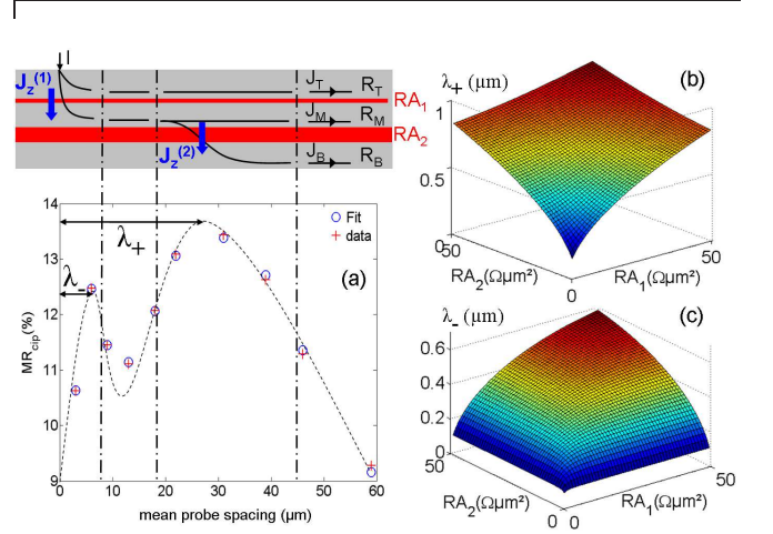
FIG. 3. (a) Comparison of Capres data with our model using RA_1 = 700\Omega\cdot\mu m^2 , RA_2 = 12.6k\Omega\cdot\mu m^2 , MR_1 = 160\% , MR_2 = 50\% , R_T = 36\Omega/\square , R_M = 69\Omega/\square , R_B = 13\Omega/\square (the dashed line is a guide for the eye); on top a sketch of the current flow (black) through the structure compared to the two length scales \lambda_+ and \lambda_- ; (b), (c) \lambda_+ and \lambda_- as a function of RA_1 and RA_2 .
