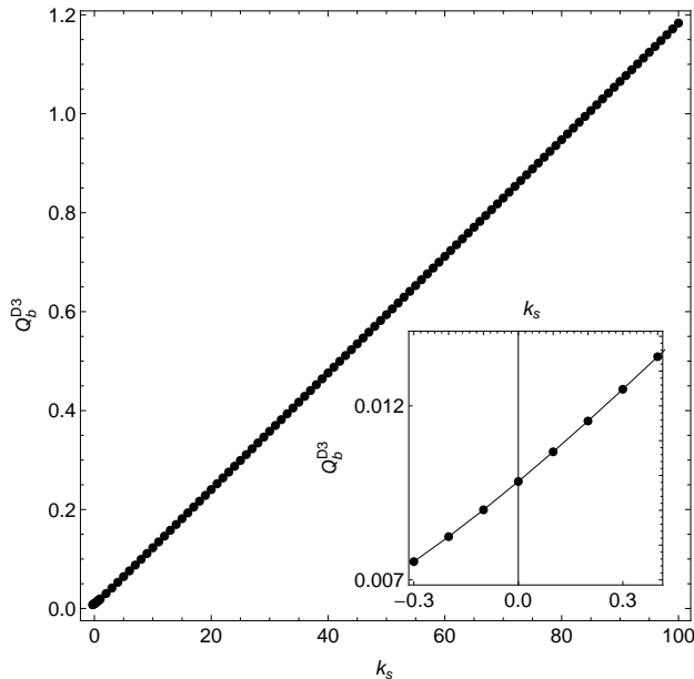
Figure 5: Mobile D3-brane charge Q_b^{D3} for mass-deformed KS black holes with mass-deformation parameters f_{a10} = 0.1 and k_{110} = 0 , as a function of k_s (related to T/\Lambda ).
