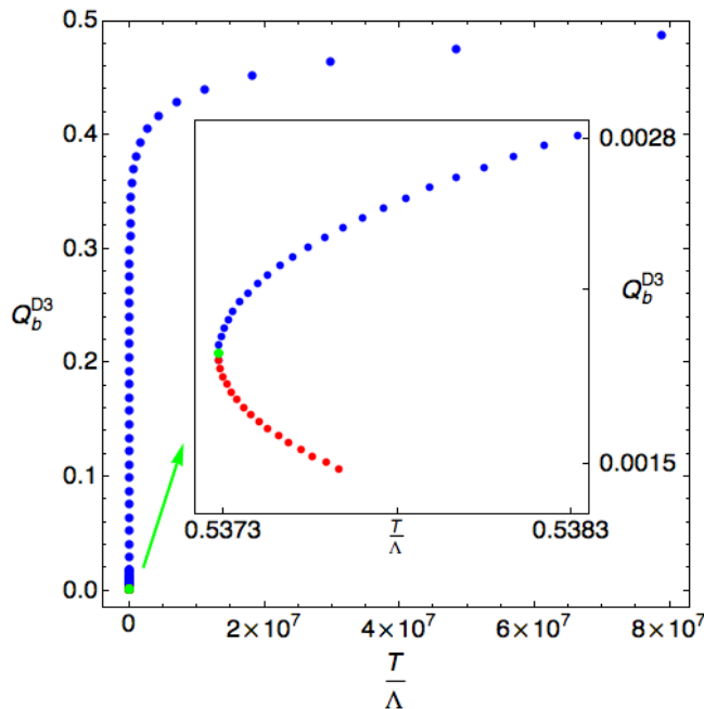
Figure 4: The dimensionless D3-brane charge of the black hole Q_b^{D3} as a function of the dimensionless temperature.
