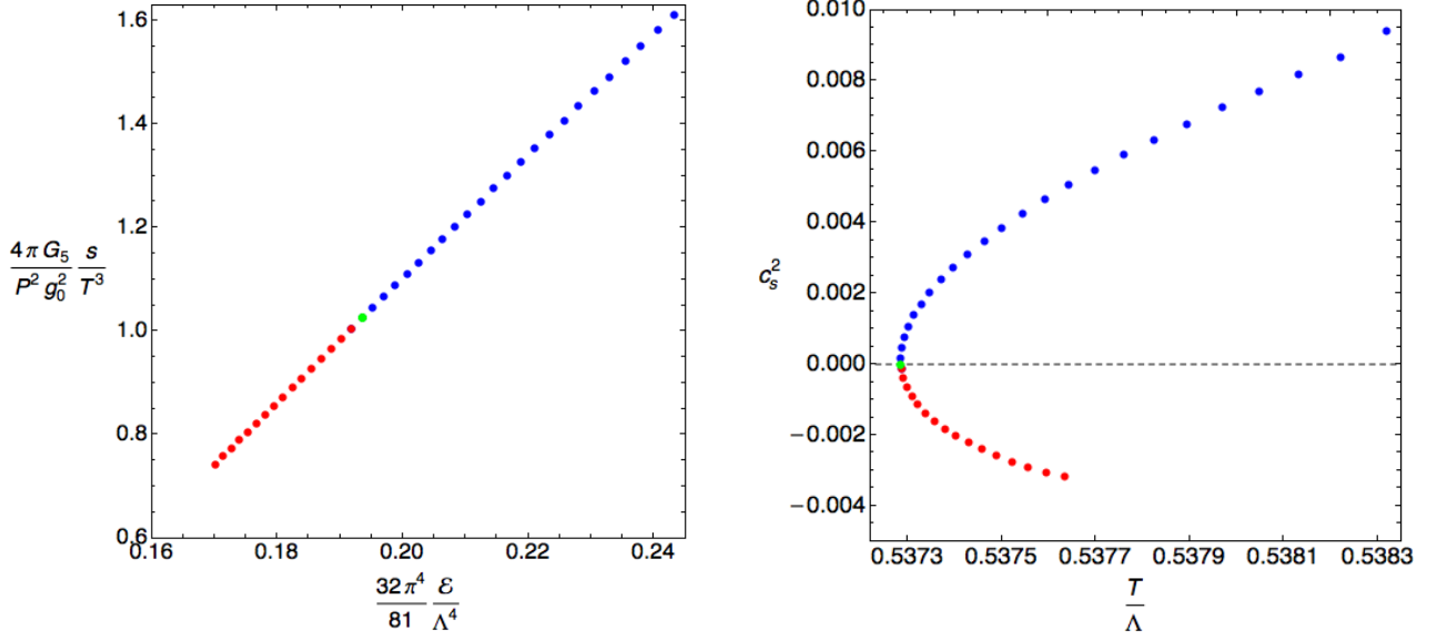
Figure 3: Left Panel: The dimensionless entropy density as a function of the dimensionless energy density in the vicinity of T = T_u . Right Panel: Square of speed of sound c_s^2 in the vicinity of T = T_u .
