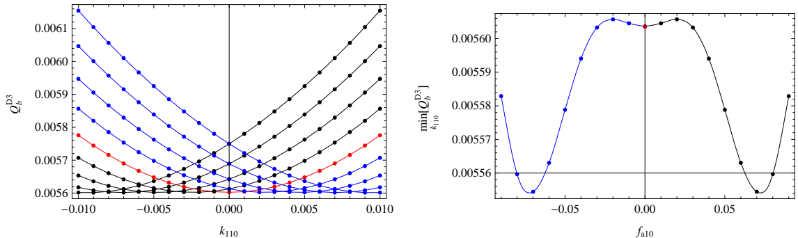
Figure 7: Same as Fig. 6, but with k_s = -0.5 .
