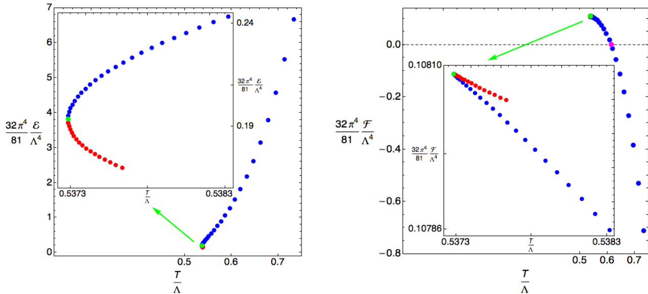
Figure 2: Left Panel: The dimensionless energy density as a function of the dimensionless temperature. The inset plot shows this energy in the vicinity of the onset of the perturbative instability of the cascading plasma (where T = T_u , the green point). Right Panel: The dimensionless free energy density as a function of the temperature for temperatures at the deconfinement transition ( T = T_c ; magenta point) and around it. The inset plot shows the free energy density in the vicinity of the perturbative instability of the cascading plasma ( T = T_u ; green point) and all the way down to the last red point that represents the last KT black hole that exists. In these figures, the red/blue dots have the same meaning as in Fig. 1.
