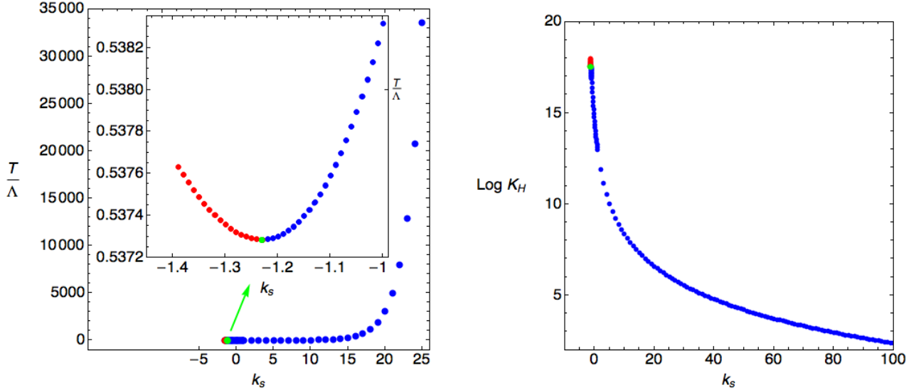
Figure 1: Left Panel: The dimensionless temperature \frac{T}{\Lambda} as a function of the microscopic parameter k_s . The inset plot zooms it in the neighbourhood of T = T_u (green point). The red dots correspond to k_s \leq k_u and the blue dots correspond to k_s \geq k_u . To the left of the last red dot there are no black holes. Right Panel: The Kretschmann scalar at the horizon as a function of the microscopic parameter k_s .
