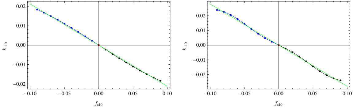
Figure 8: Relation between the mass-deformation parameters f_{a10} and k_{110} for k_s = 0 ( Left Panel ) and k_s = -0.5 ( Right Panel ) at \min Q_b^{D3} . The solid green lines represent the best fit linear relation f_{a10} \propto k_{110} .
