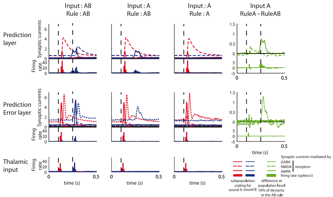
Figure 7. Simulating the MMN to the omission of an expected sound. First column, Mean response to a frequent AB pair. The network learns the predictable local transition A \rightarrow B , which results in a reduced response to the predictable B sound (see arrow). Second column, Mean response to a rare A sound presented in isolation in the same context. The network generates a response to the omission of the expected sound B (arrow). Third column, Response to the same isolated sound A, in a different context where it is the frequent stimulus. Although the stimulus is physically identical to the second column, the predictive response to the omitted B sound is no longer seen. Fourth column, Difference between the second and third columns, isolating the simulated MMN to omission.
