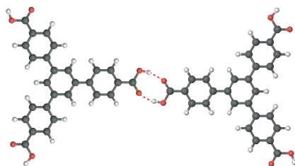
Figure 1: Scheme of hydrogen-bonded 1,3,5-Tris(4-carboxyphenyl)benzene ( C_{27}H_{18}O_6 ) dimer. Carbon atoms are gray, oxygen atoms red, hydrogen atoms white, respectively. Red dotted lines represent molecular hydrogen bonds.
