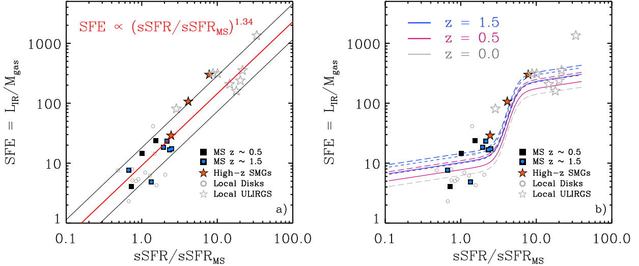
FIG. 9.— a) Star formation efficiency, SFE = L_{\text{IR}}/M_{\text{gas}} , against the offset from the main sequence. Black squares and orange stars are the MS galaxies and the SMGs considered in this study. Empty grey circles are local normal galaxies (Leroy et al. 2008 and Schrubba et al. 2012) and grey stars depict local ULIRGs (Zaurin et al. 2009 and Solomon et al. 1997). For local ULIRGs we have assumed ( \alpha_{\text{CO}} = 0.8 ). The red solid line depicts the best fit to the data with a slope of 1.34, while a Spearman’s rank test indicates a tight correlation between the plotted quantities with \rho = 0.71 . b) Same as the left panel but for the case of a weak increase of SFE with s\text{SFR}/s\text{SFR}_{\text{MS}} within the main sequence. Tracks show the dependence of SFE on s\text{SFR}/s\text{SFR}_{\text{MS}} as expected for a slightly sub-linear relation between M_{\text{gas}} and SFR and the relative importance of the starburst and main-sequence mode of star formation as a function of s\text{SFR}/s\text{SFR}_{\text{MS}} . Blue (purple), solid, dashed and long-dashed lines correspond to z = 1.5 ( z = 0.5 ) for M_* = 1.0 \times 10^{10} M_{\odot} , 5.0 \times 10^{10} M_{\odot} , and 1.0 \times 10^{11} M_{\odot} . Grey long-dashed line corresponds to z = 0 and M_* = 1.0 \times 10^{11} M_{\odot} .
