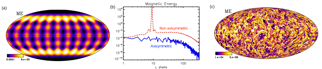
Figure 5. (a) Initial magnetic energy (the seed poloidal streamfunction is a l = 9, m = 5 spherical harmonic) in cgs, in the middle of the convection zone. (b) Magnetic energy spectra one timestep after the introduction of the peaked magnetic field in our turbulent convection zone. The axisymmetric spectra are in plain blue, the non-axisymmetric spectra in dashed red, and the total spectra in dotted black. (c) Saturated magnetic energy in cgs, 600 days after the introduction of the seed magnetic field. The color scale is logarithmic.
