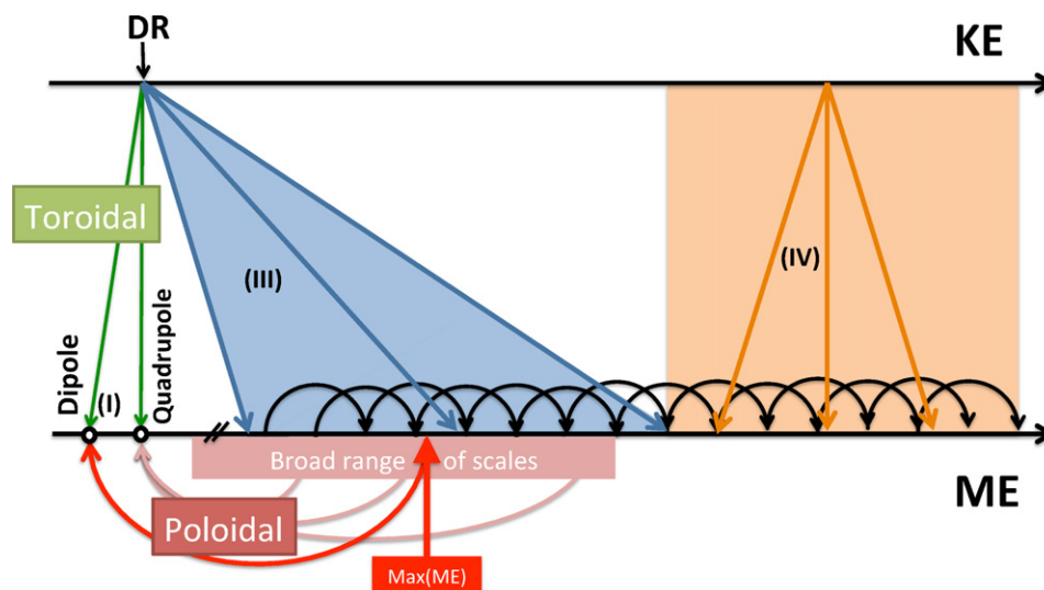
Figure 14. Saturating interactions of the nonlinear convective dynamo summarizing the results of Section 4. KE and ME stand for kinetic and magnetic energy and DR for differential rotation.
