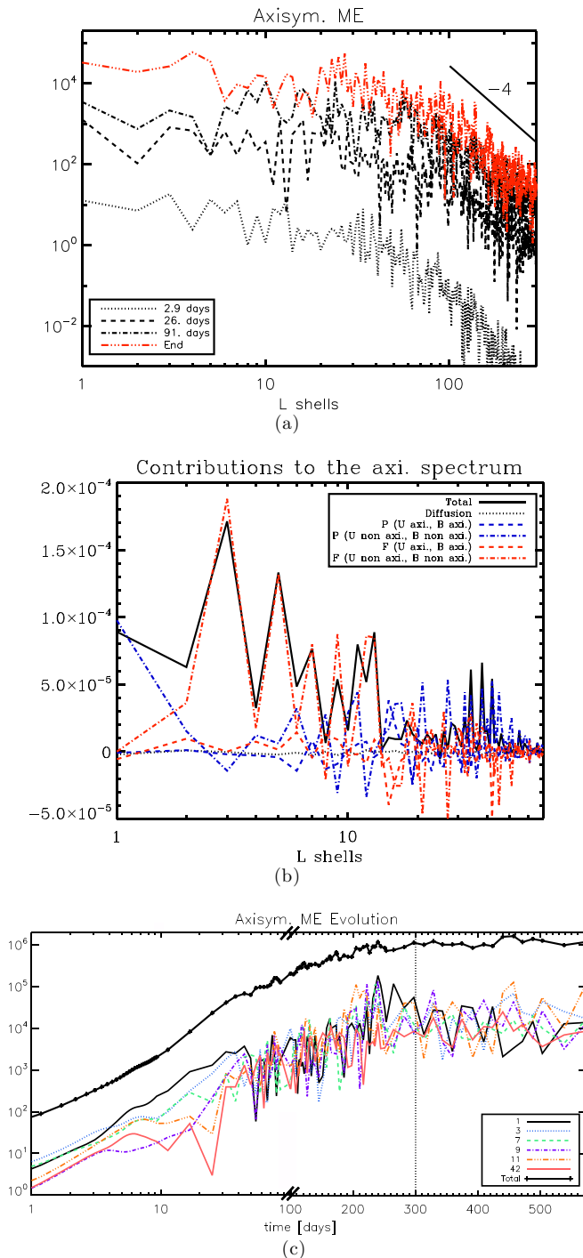
Figure 9. Same as for Figure 6, but for the axisymmetric part of the spectrum. In panel (a), the initial spectrum is zero.
