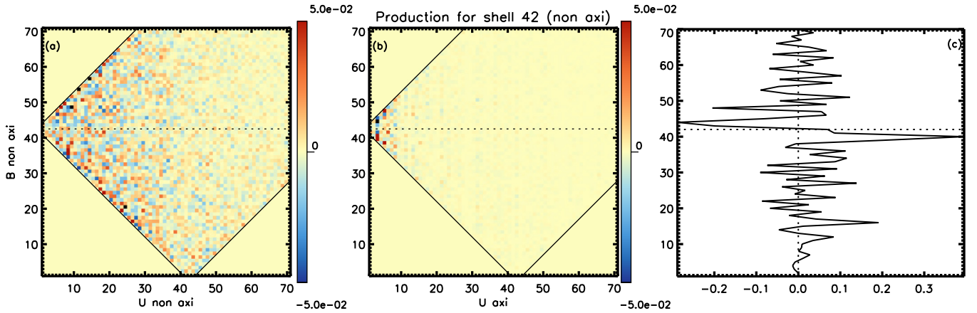
Figure 11. Production \mathcal{P} contribution to the non-axisymmetric shell L = 42 during the saturation phase. Interactions between \mathbf{B}^0 and \mathbf{U}^* are negligible.
