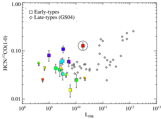
Figure 6. HCN/ ^{12}\text{CO}(1-0) versus FIR luminosity. Early-type galaxies are shown as colored squares with the color reflecting their \mathcal{R}_{10} ratio (blue to red depicts low to high ratios). Late-type galaxies from the Gao & Solomon (2004b) sample are shown as diamonds. NGC 1266 is highlighted by a surrounding circle.
