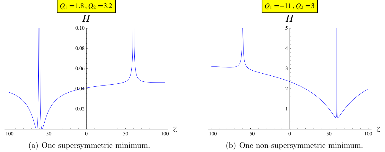
Figure 3: A single stable minimum between the two centers. When both charges are positive and have the same orientation as the background (which has electric potential Z > 0 at the left center), the minimum is supersymmetric. When one of the charges has the wrong orientation, the minimum is non-supersymmetric. Note that the apparent second minimum outside the 2-center range is connected to the one inside by a Mexican-hat-type potential around the center in the z - \rho plane. As we will show below in fig. 7, when supersymmetry is broken this Mexican-hat potential is slightly tilted.
