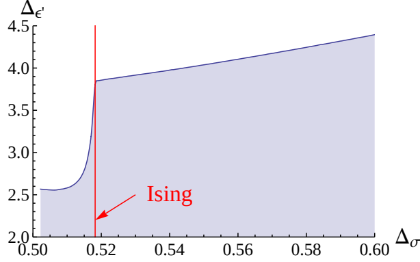
Figure 6: The bound on \Delta_{\varepsilon'} under the condition that \Delta_{\varepsilon} has already been fixed to the maximal value allowed by Fig. 3. Here n_{\max} = 10 (see Appendix D). The width of the vertical red line marking the 3D Ising value of \Delta_{\sigma} is about five times the error band in Table 1.
