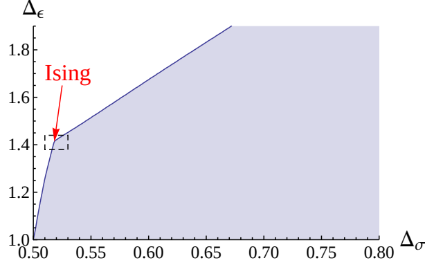
Figure 3: Shaded: the part of the (\Delta_\sigma, \Delta_\epsilon) plane allowed by the crossing symmetry constraint (5.3). The boundary of this region has a kink remarkably close to the known 3D Ising model operator dimensions (the tip of the arrow). The zoom of the dashed rectangle area is shown in Fig. 4. This plot was obtained with the algorithm described in Appendix D with n_{\max} = 11 .
