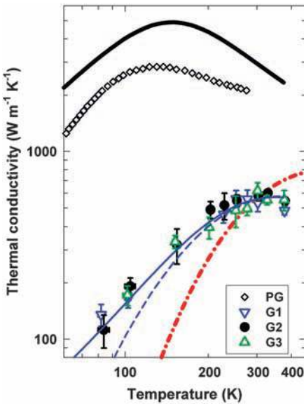
Fig. 4. Measured thermal conductivity of G1, G2, and G3 together with the highest reported values of PG (5), the BTE calculation results of suspended SLG (black solid line) and supported SLG with K_{\text{LATA}} = 0 and K_{\text{ZA}} = 0.73 N/m (blue solid line) or K_{\text{LATA}} = K_{\text{ZA}} = 0.46 N/m (blue dashed line), the RTA calculation result (red dashed-dotted line) for supported SLG with K_{\text{LATA}} = 0.8 N/m. Specular edges are assumed in the calculations. For supported SLG, s = d = 30 nm, and the calculation results are insensitive to edge specularity and can be reproduced with decreased d/s and increased K_{\text{ZA}} for the same K_{\text{LATA}}/K_{\text{ZA}} .
