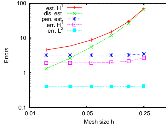
FIGURE 9. Actual errors in H^1(\Omega) and L^2(\Omega) norms, total estimator, discretization estimator and penalization estimator for the velocity for \varepsilon = 10^{-1} .
