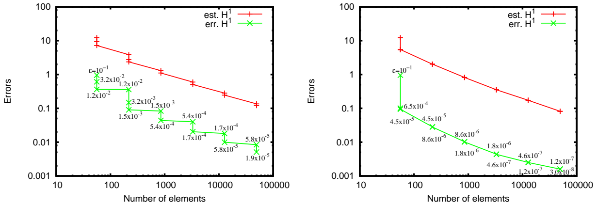
FIGURE 10. Actual errors in H^1(\Omega) and total estimator for the velocity. Left: \gamma = 1/10 , right: \gamma = 1/500 .
