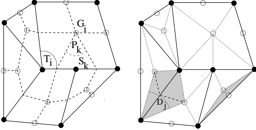
FIGURE 1. A non-conforming primal mesh (solid lines) and its associated dual mesh (left, dashed lines) and diamond mesh (right, dotted lines).
