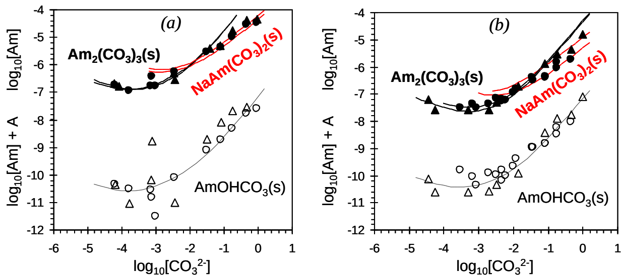
Figure 4. Solubility of Am(III), [\text{Am}] , in bicarbonate and carbonate solutions with 4 mol/L NaCl measured (●) in phase 1 (cooling) and (▲) in phase 2 (heating) for (a) T = 30^\circ\text{C} and (b) T = 70^\circ\text{C} . The slope analysis suggests that (—) \text{Am}_2(\text{CO}_3)_3(\text{s}) and (—) \text{NaAm}(\text{CO}_3)_2(\text{s}) control the solubility. In the case \text{AmOHCO}_3(\text{s}) would control the solubility, \log[\text{Am}] + A is represented (open symbols, dashed line is a guide to the eye), where A = -0.5 \log_{10} P_{\text{CO}_2} + 0.5 \log(K_w^2 K_{p2}) , \log_{10} K_w = -14.17 ( K_w is the ionic product of water at the considered ionic strength) and \log_{10} K_{p2} = 17.70 ( K_{p2} is the equilibrium constant for \text{CO}_3^{2-} + 2 \text{H}^+ \rightleftharpoons \text{CO}_2(\text{g}) + \text{H}_2\text{O} ) (Reprinted with permission from Vercouter et al., 2005a. Copyright 2005 American Chemical Society).
