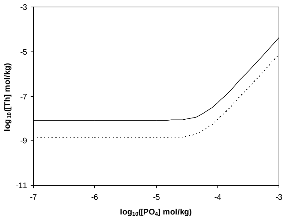
Figure 12. Effect of the Th(HPO_4)_{n^{4-2n}} complexes proposed in Ekberg et al. (2010), and extrapolated in Table 2 on the solubility at pH 8 and I = 0.1 mol NaClO_4/L of ThO_2(am,hyd,aged) (dotted) and ThO_2(am,hyd,fresh) (plain) from Rand et al. (2009).
