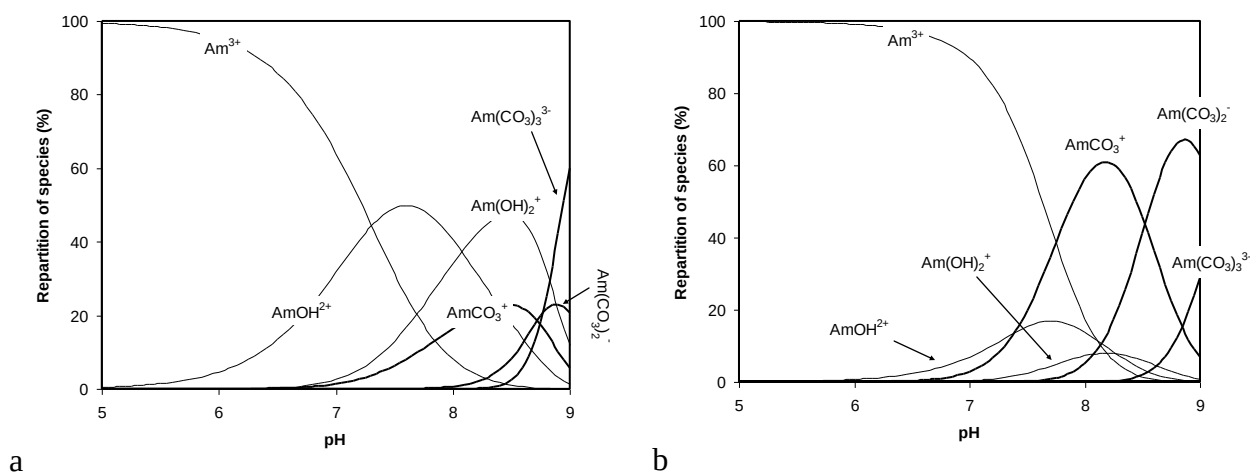
Figure 3. Differences induced in the speciation diagram of trace Am(III) at I = 1 \text{ mol/L} , and p\text{CO}_2 = 10^{-3.46} \text{ atm} , between values selected in Silva et al. (1995) (left) and Guillaumont et al. (2003) (right).
