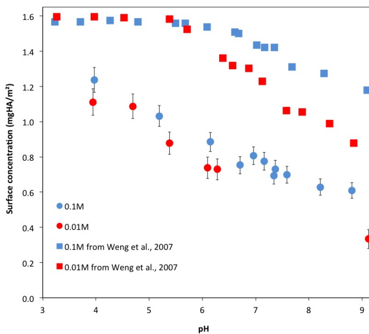
Figure 1. Influence of pH and ionic strength on PAHA adsorption onto \alpha -Al 2 O 3 . Re-calculated data from Weng et al. (2007) for HA adsorption onto goethite have been plotted for comparison.
