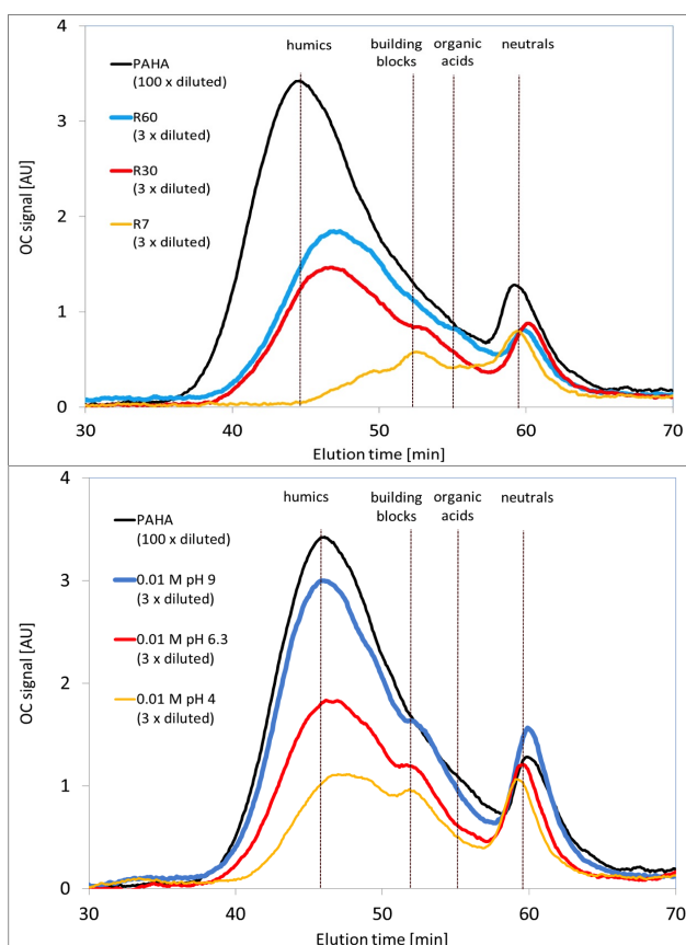
Figure 3. LC-OCD chromatograms of PAHA and of supernatants from adsorption experiments (A, top) at 0.1 M and pH \approx 6.8 ( R in mg PAHA /g \alpha -Al 2 O 3 ) and (B, bottom) at 0.01 M and different pH ( R \approx 25 mg PAHA /g \alpha -Al 2 O 3 ).
