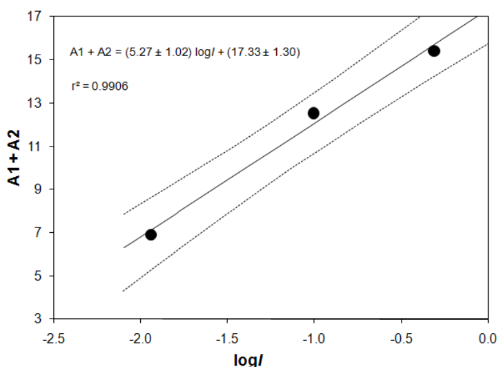
Figure 4. Comparison of the evolution of maximal absorbance A_1 + A_2 as a function of \log I . The continuous line is the result of the linear regression and the dotted ones the statistical envelope (A_1 + A_2) \pm \sigma(A_1 + A_2) .
