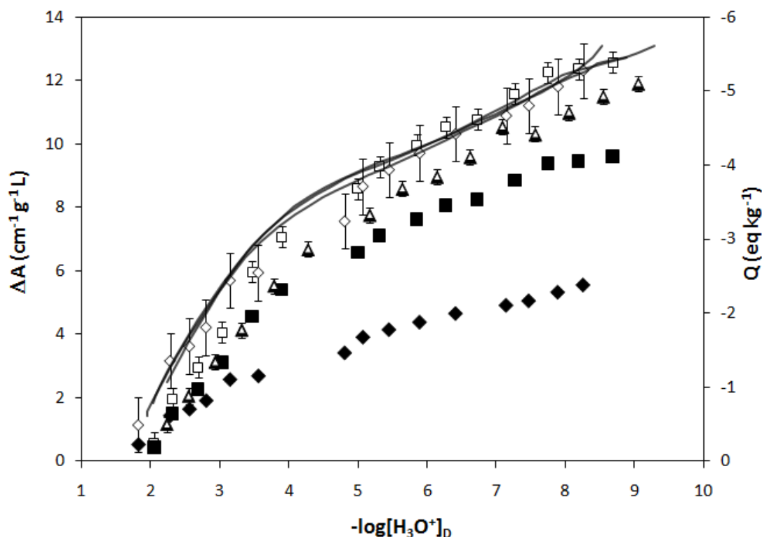
Figure 3. Original and corrected spectrophotometric titration curves of PAHA at I = 0.01 ( \diamond ), 0.1 ( \square ), and 0.5 ( \triangle ) \text{mol/L NaClO}_4 .
