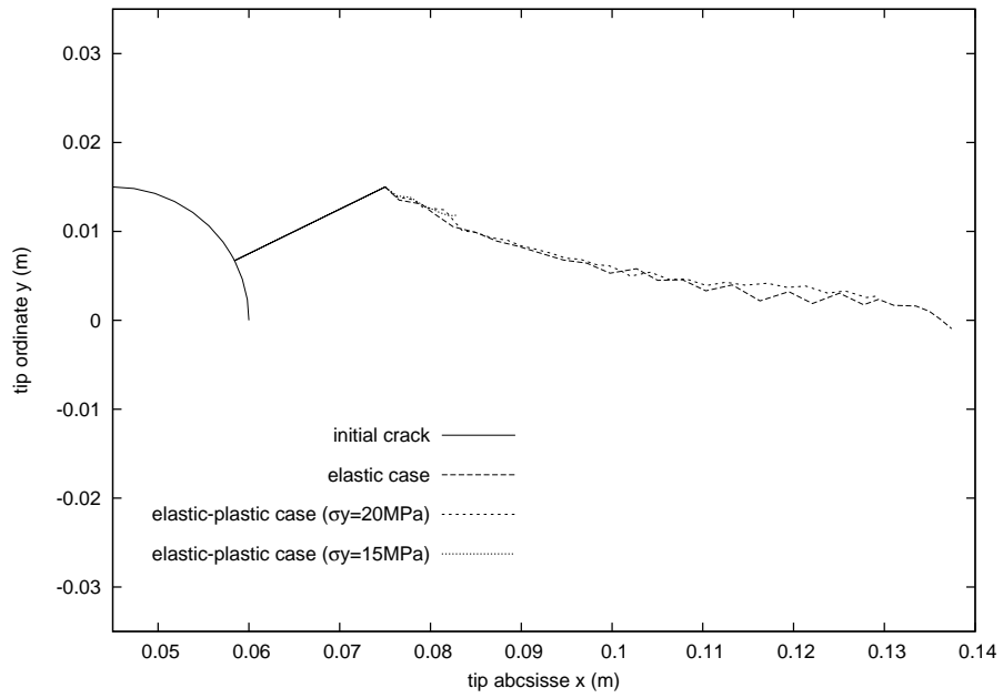
Figure 15: Crack path
