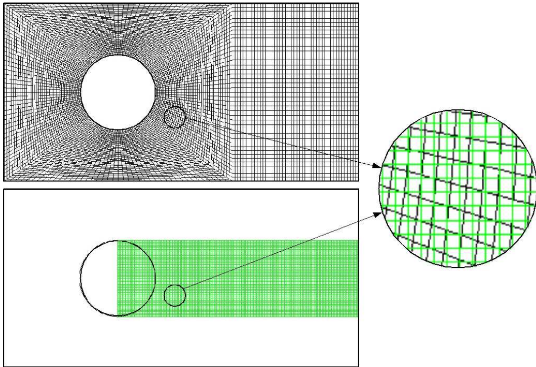
Figure 7: Unstructured mechanical mesh (top), regular level set grid (bottom)
