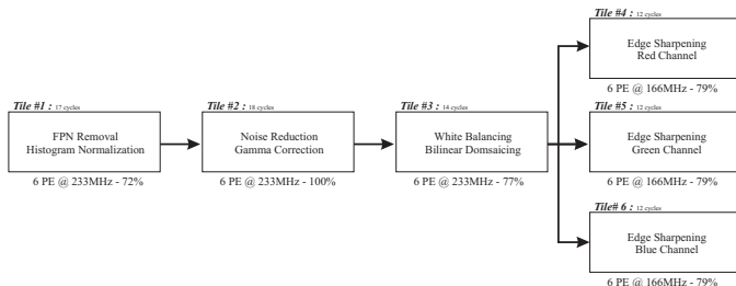
Fig. 3. Algorithms arrangement on the different computing tiles.
