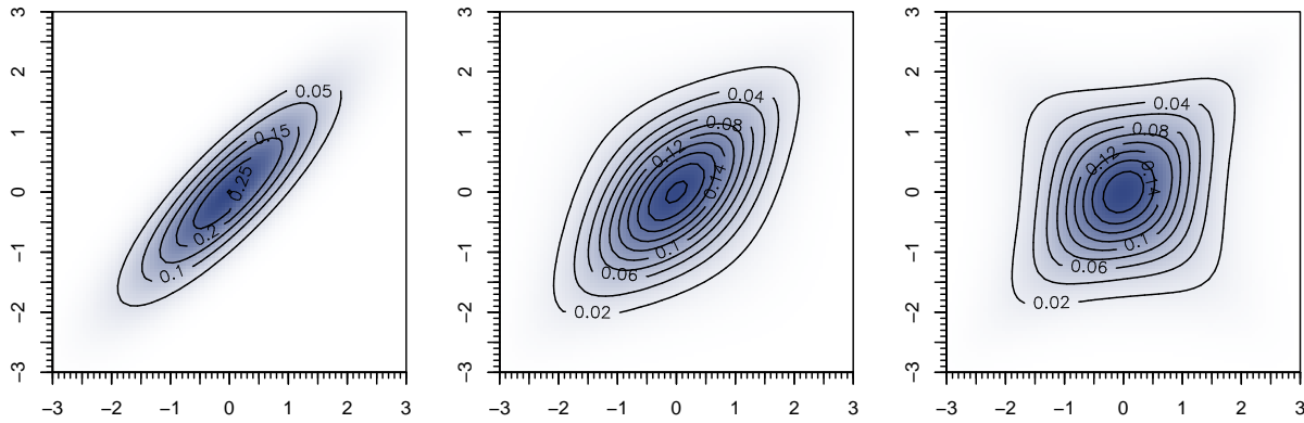
Fig. 3. Probability density functions of different t-copulas with \rho=0.85 and \nu=\infty, 5, 2.5 respectively (from left to right). For better comparability, the marginal distributions are chosen to be standard normal.
