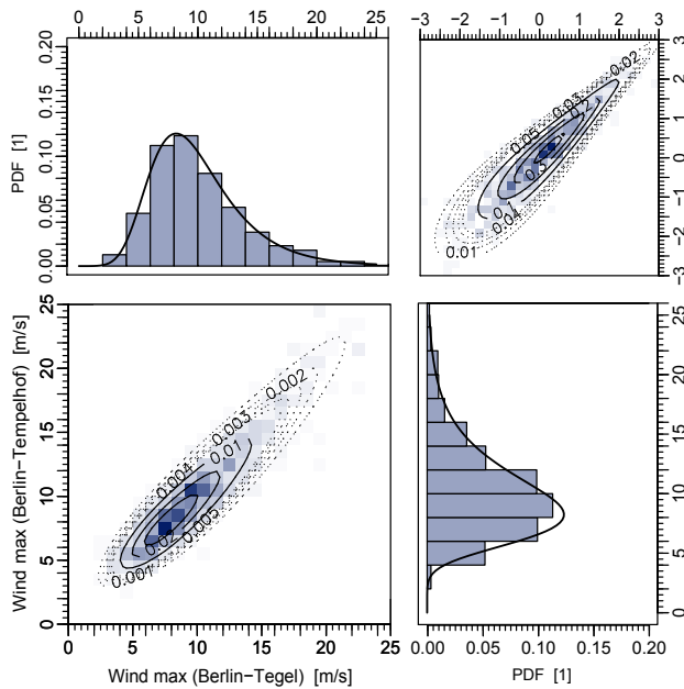
Fig. 7. Bivariate distribution of daily wind maxima at station Berlin-Tegel and Berlin-Tempelhof (see text and Fig. 5). The parameter estimates (and standard errors) of the GEV distribution, and the Gumbel copula are \hat{\mu}_{\text{Teg}}=8.24 (0.12), \hat{\sigma}_{\text{Teg}}=3.05 (0.09), \hat{\xi}_{\text{Teg}}=0.021 (0.026), \hat{\mu}_{\text{Tem}}=8.41 (0.088), \hat{\sigma}_{\text{Tem}}=2.98 (0.09), \hat{\xi}_{\text{Tem}}=0.059 (0.027), and \hat{\theta}_G=4.09 (0.12).
