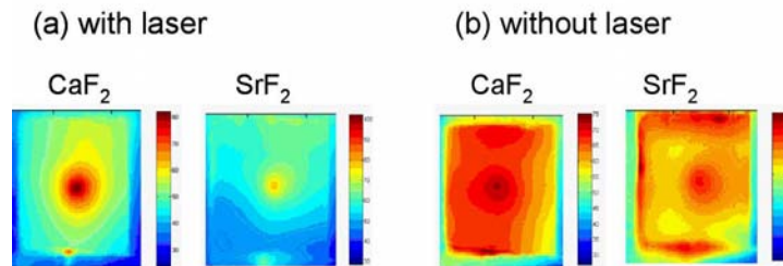
Fig. 3. Thermography of \text{Yb}^{3+}:\text{CaF}_2 and \text{Yb}^{3+}:\text{SrF}_2 (a) with laser operation and (b) without laser operation at maximum pump power. The cooled sides are right left and bottom.
