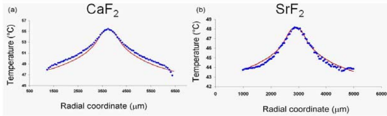
Fig. 7. Experimental (bleu points) and the corresponding theoretical (red line) temperature profiles at z=0 for (a) \text{Yb}^{3+}:\text{CaF}_2 and for (b) \text{Yb}^{3+}:\text{SrF}_2
