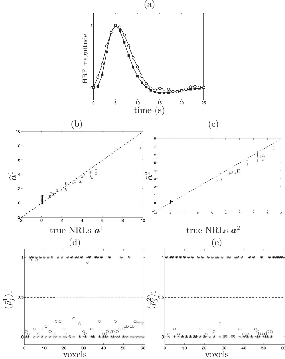
Fig. 2. Estimation results on the simulated data using model \mathcal{M}_1 . (a) HRF results: Symbols \blacksquare and \circ represent the true h_c and its corresponding HRF estimate, respectively. (b)-(c): NRL estimates for conditions 1 and 2, respectively. True values appear on the x -axis and estimated values on the y -axis. The error bars follow Eq. (10). (d)-(e): PM estimates of activation probabilities \hat{p}_j^m ( \circ symbols) for the conditions 1 and 2, respectively. Symbols * depict the true class attached to each voxel.
