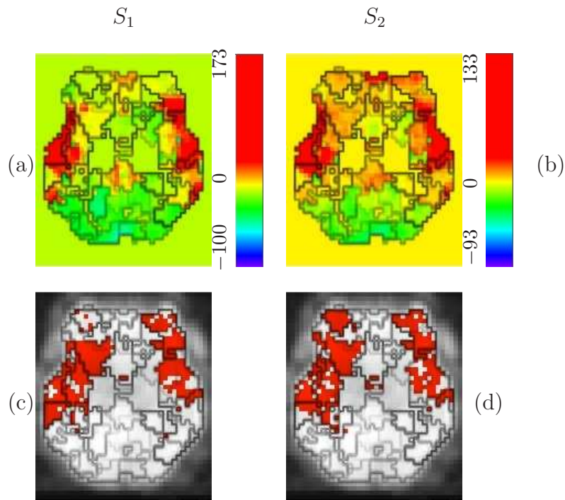
Fig. 10. (a)-(b) NRL estimates in one slice of subject 1’s brain (at z = -4 mm) in response to S_1 (a) and S_2 (b). Values correspond to the NRL coefficients only for voxels belonging to \mathcal{M}_s . Otherwise they are equal to 0. (c)-(d) : detection results in the same slice for S_1 and S_2 , respectively. Voxels colour-coded in red are detected as activating. In black are the parcel borders that are superimposed to the different map results to show the parcellisation influence on the estimation of such parameters.
