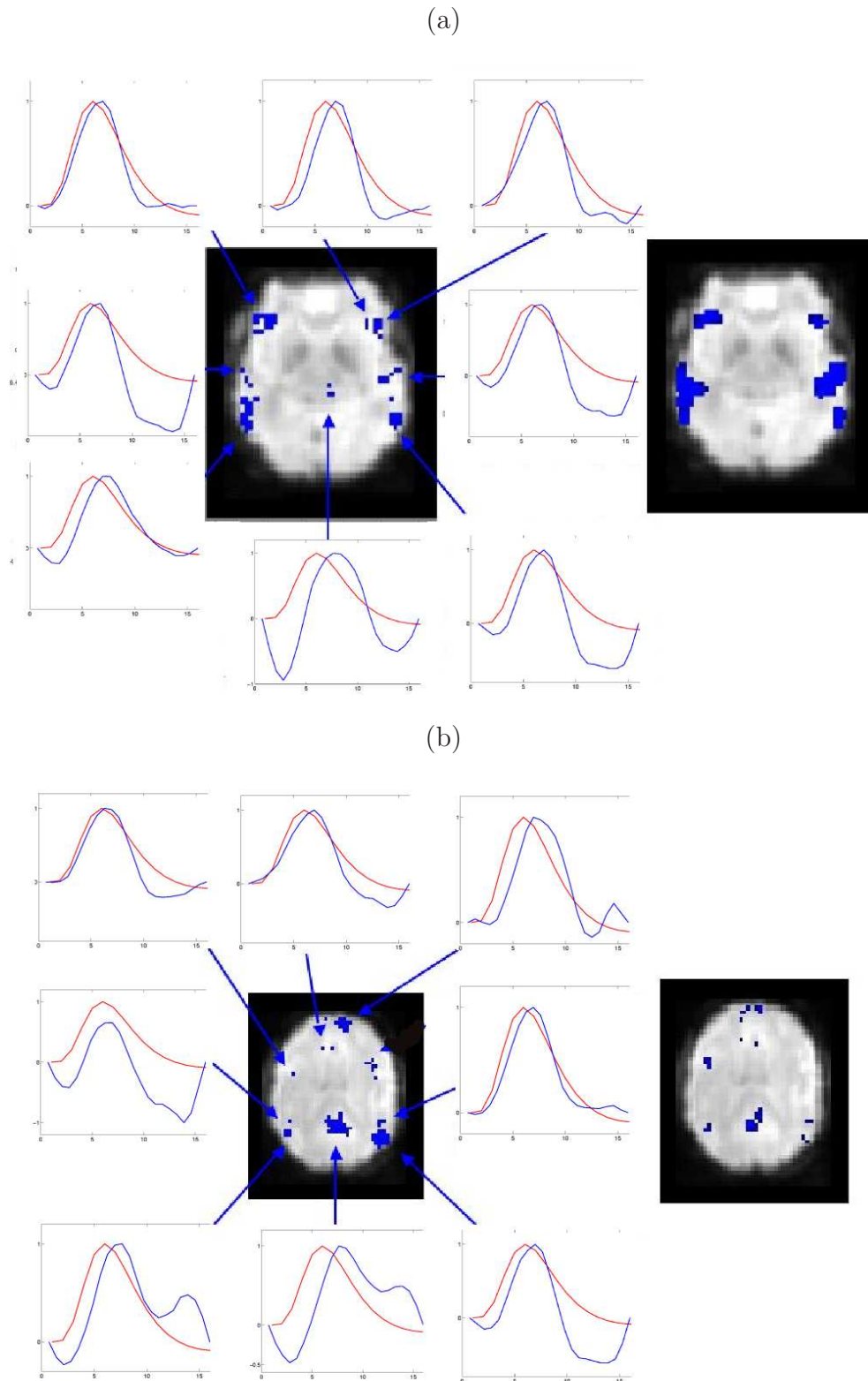
Fig. 14. (a) : Single-slice comparison ( z = 0 mm, slice 7 in Fig. 13) for the contrast S_1 > S_2 . left panels : thresholded PPM at \eta = 0.999 ; right panels : thresholded SPM t-map at T=3.09 (corrected for multiple comparisons) obtained from the SPM analysis. (b) : same comparison in slice z = 24 mm (slice 13 in Fig. 13). HRF estimates (in blue) in these regions compared to the canonical hemodynamic response function used in SPM (in red).
