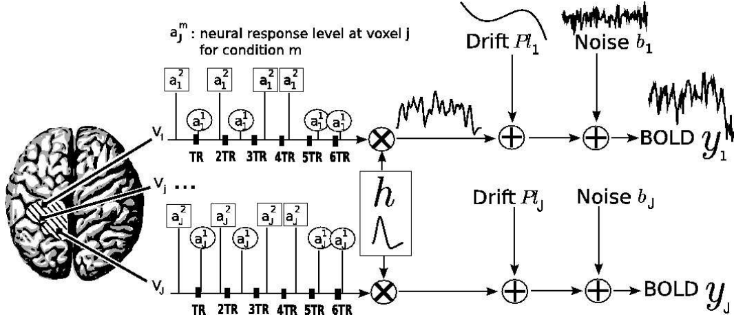
Fig. 1. Summary of the proposed regional BOLD model. The size of each parcel \mathcal{P} varies typically between by a few tens and a few hundreds: 80 \leq J \leq 350 . The number M of experimental conditions involved in the model usually varies from 1 to 5. In our example, M = 2 , the NRLs ( a_j^1, a_j^2 ) corresponding to the first and the second conditions are surrounded by circles and squares, respectively. Note that our model accounts for asynchronous paradigms in which the onsets do not necessarily match acquisition time points. As illustrated, the NRLs take different values from one voxel to another. The HRF h can be sampled at a period of 1s and estimated on a range of 20 to 25s (e.g., D = 25 ). Most often, the LFD coefficients \ell_j are estimated on a few components ( Q = 4 ).
