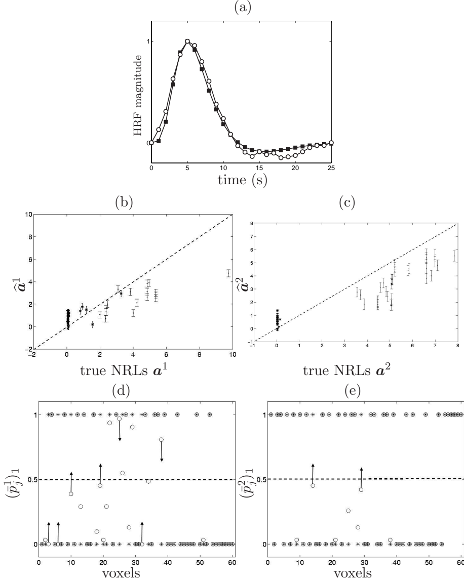
Fig. 5. Simulation results using model \mathcal{M}_4 . The same legend as in Fig. 2 holds. FP and FN voxels are indicated by downward and upward arrows, respectively.
