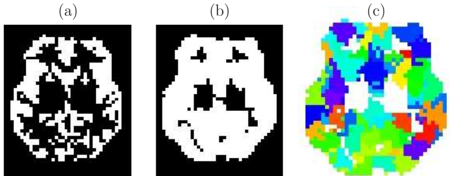
Fig. 9. (a): Slice of Subject 1’s anatomical mask ( z = -4 mm). (b): its dilated version \mathcal{M}_a to match the functional resolution. (c): corresponding parcellation in the same slice. Each colour codes for a different parcel.
