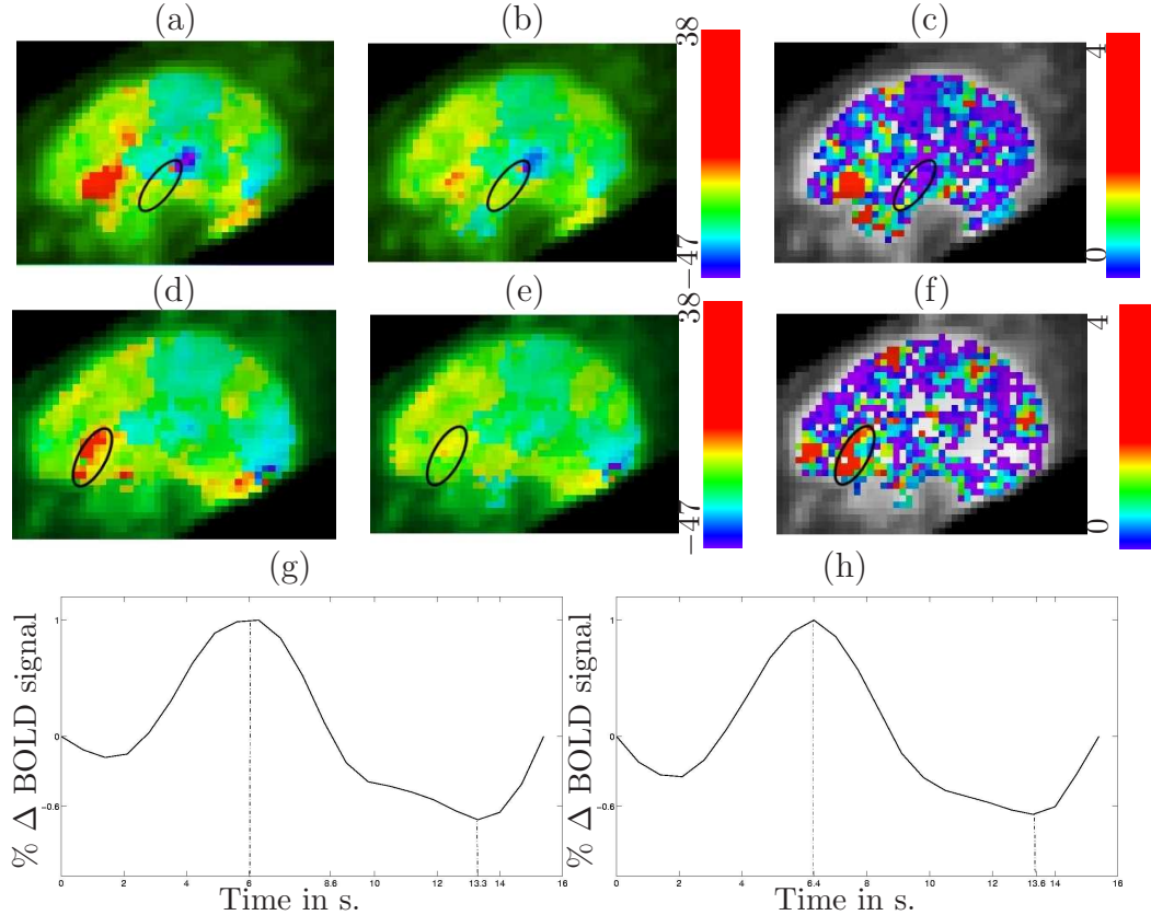
Fig. 15. (a)-(b) & (d)-(e): NRL estimates in the sagittal slices located at x = -48 mm and x = -40 mm, respectively. (a)-(b) provide the magnitudes in response to S_1 while (d)-(e) give us the NRLs in response to S_2 . (c)-(f): KL-distance maps between the corresponding NRLs. Images are superimposed to functional data. The parcels containing the Heschl's gyrus (top row) and Broca's area (bottom row) are surrounded in black and referenced as \mathcal{P}_{He} and \mathcal{P}_{Br} in the text. (g)-(h): HRF estimates in \mathcal{P}_{He} and \mathcal{P}_{Br} , respectively.
