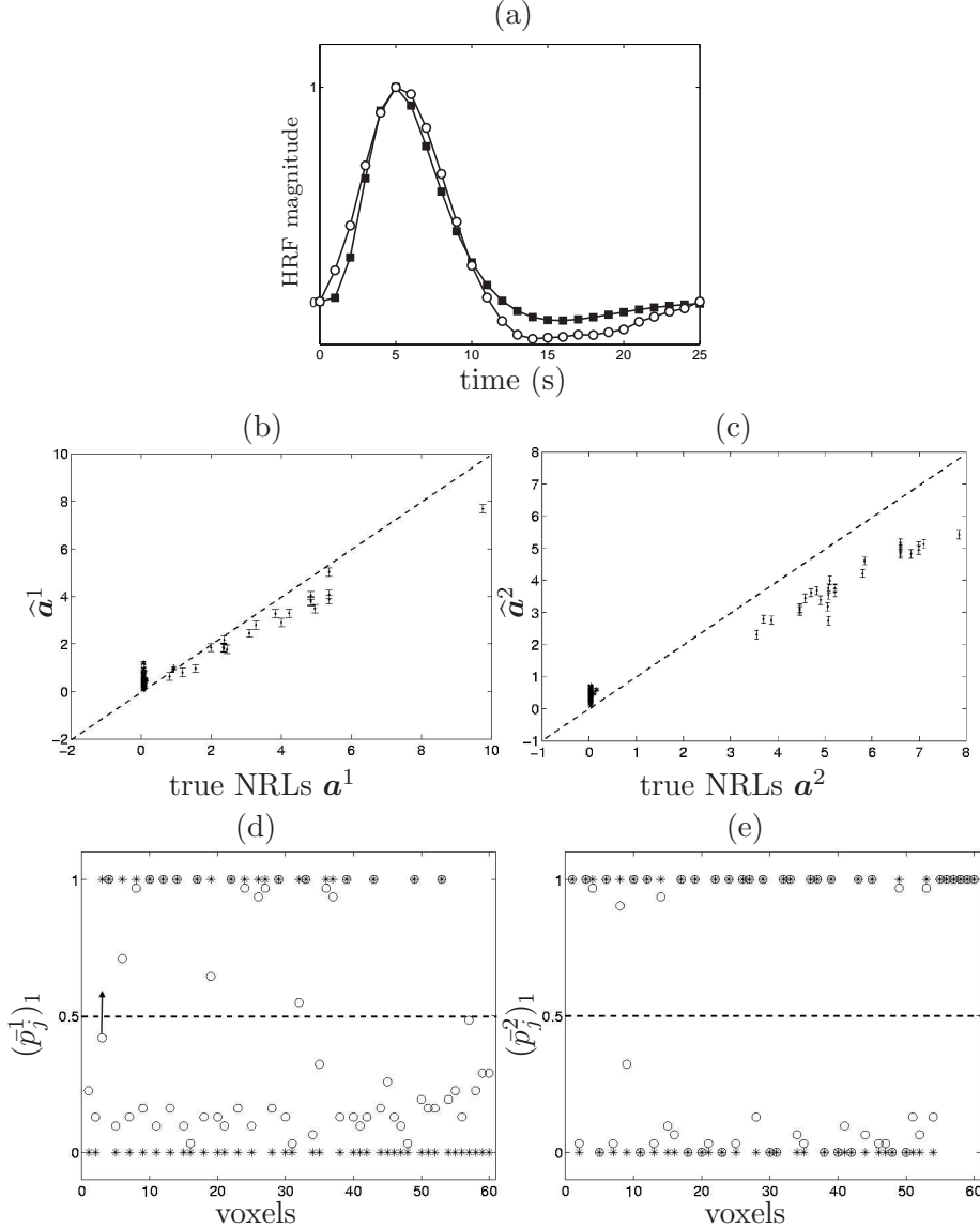
Fig. 3. Simulation results using model \mathcal{M}_2 . The same legend as in Fig. 2 holds. Only one FN voxel is present, indicated with an upward arrow.
