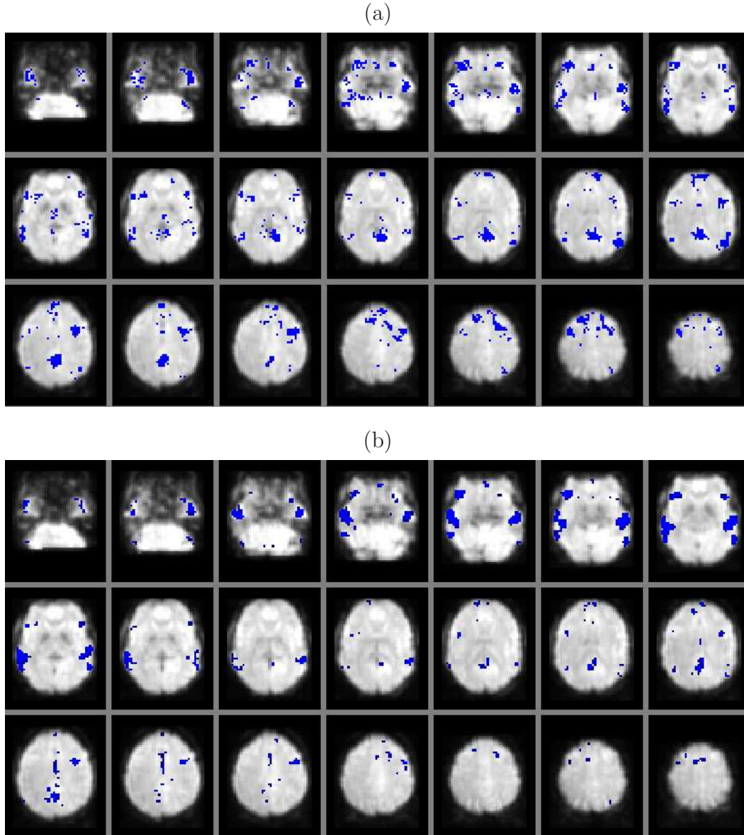
Fig. 13. From left to right and from top to bottom, brain slices organised along increasing axial axis (the bottom of the brain appear first in the superior left corner). Study of the contrast S_1 > S_2 . (a) : thresholded PPM (see (11)) at \eta = 0.999 ; (b) : thresholded SPM t-map at T=3.09 (corrected for multiple comparisons) obtained using SPM2.
