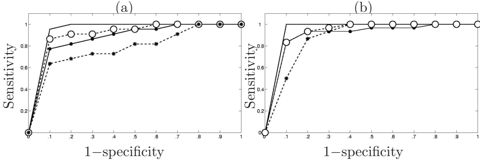
Fig. 6. (a)-(b): ROC curves associated to the four different models for condition 1 (a) and condition 2 (b), respectively. Continuous line, interrupted line with \circ , continuous line with \bullet and interrupted line with * represent the ROC curves for models \mathcal{M}_1 - \mathcal{M}_4 , respectively.
