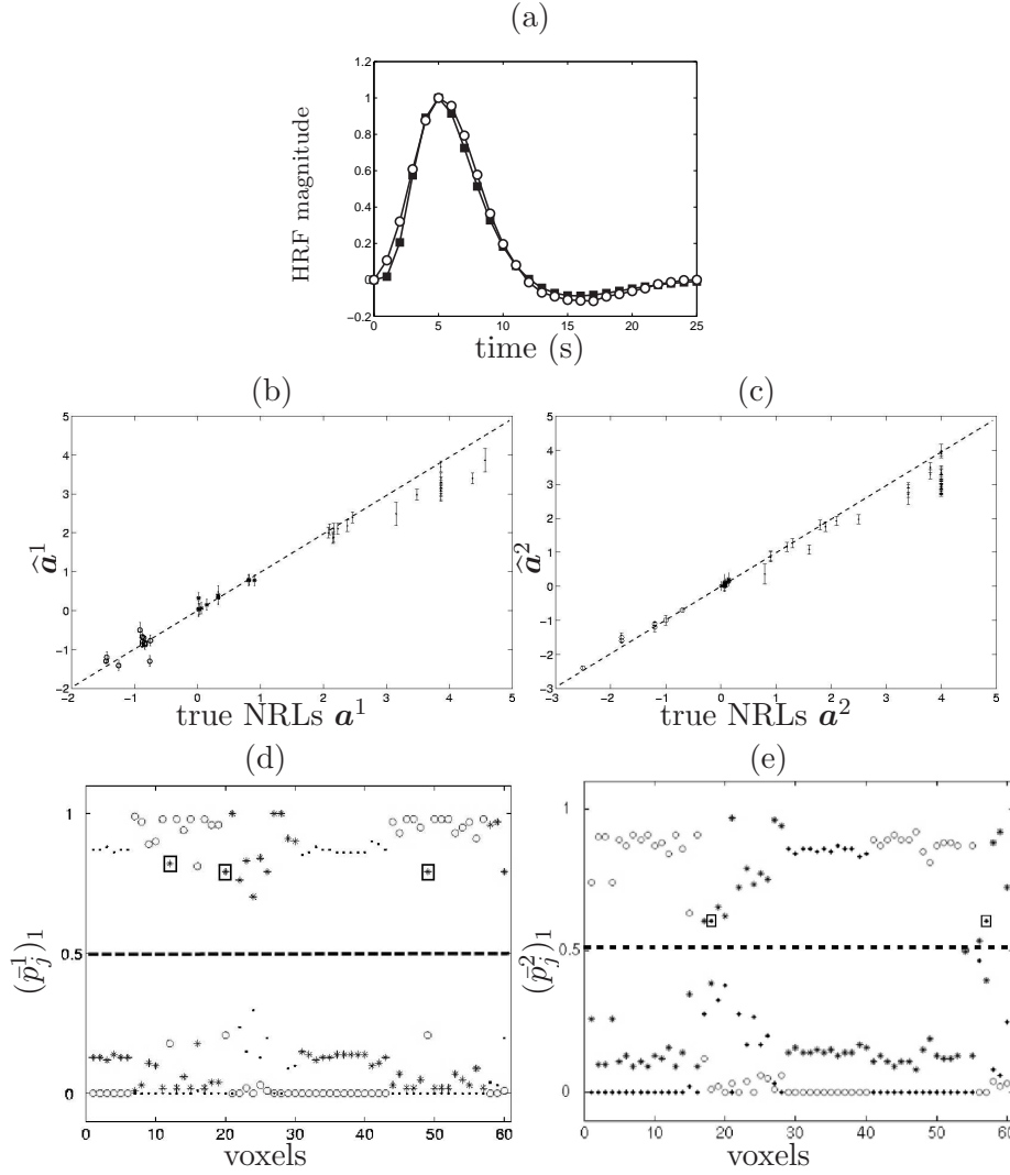
Fig. 8. Simulation results using model \mathcal{M}_5 . The same legend as in Fig.2 holds. FP and FN voxels are surrounded by rectangles (3 FNs in (d) and 2 FPs in (e)). \circ , \cdot and * symbols represent (\bar{p}_j^m)_1 , (\bar{p}_j^m)_{-1} and (\bar{p}_j^m)_0 , respectively.
