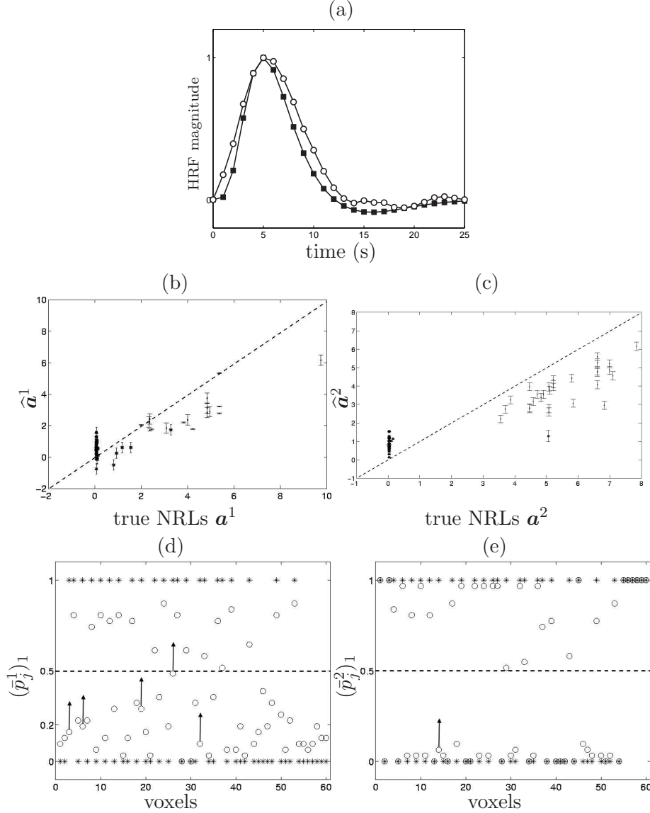
Fig. 4. Simulation results using model \mathcal{M}_3 . The same legend as in Fig. 2 holds. FN voxels are indicated by upward arrows.
