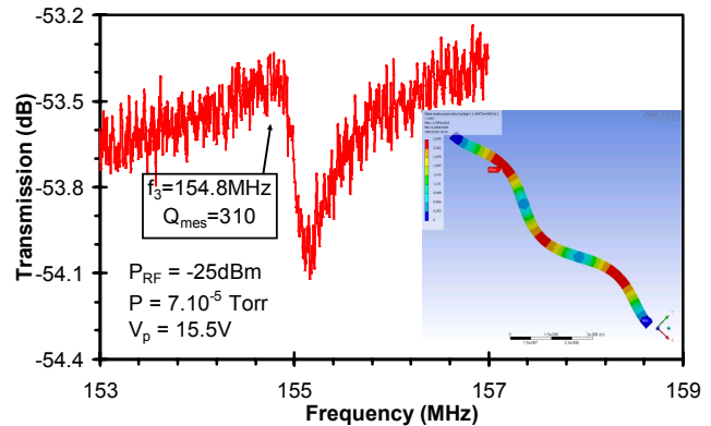
Figure 8: Frequency response showing the third resonance mode of a clamped-clamped beam resonator ( L=10\mu\text{m} , w=0.35\mu\text{m} and d=115\text{nm} )
