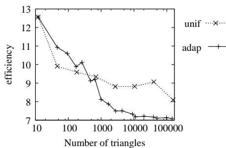
FIG. 7.6. Efficiencies for the singular solution for a uniform and an adaptive refinement.
