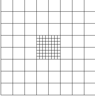
FIG. 6.1. Nonconforming mesh with h = 1/4 and p = 2 .
