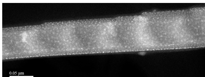
Figure 4. HAADF STEM image of a Si/SiGe nanowire. The SiGe layers are bright and the Si layers are dark.
