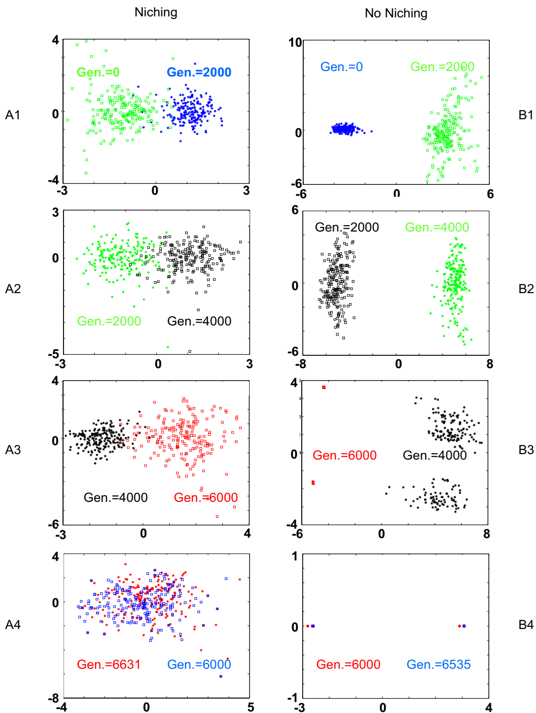
Figure 1 Evolution of the EA for a genetic algorithm with link-recombination. These figures show the evolution of the population distribution during the learning process using link-recombination with niching (A1-A4) and without niching (B1-B4). The populations were recorded every 2000 generations and after the algorithm's convergence. Each plot represents the graphs of two populations sampled consecutively. The graphs of both populations are represented as points on a 2D map using Kernel Principal Component Analysis .
