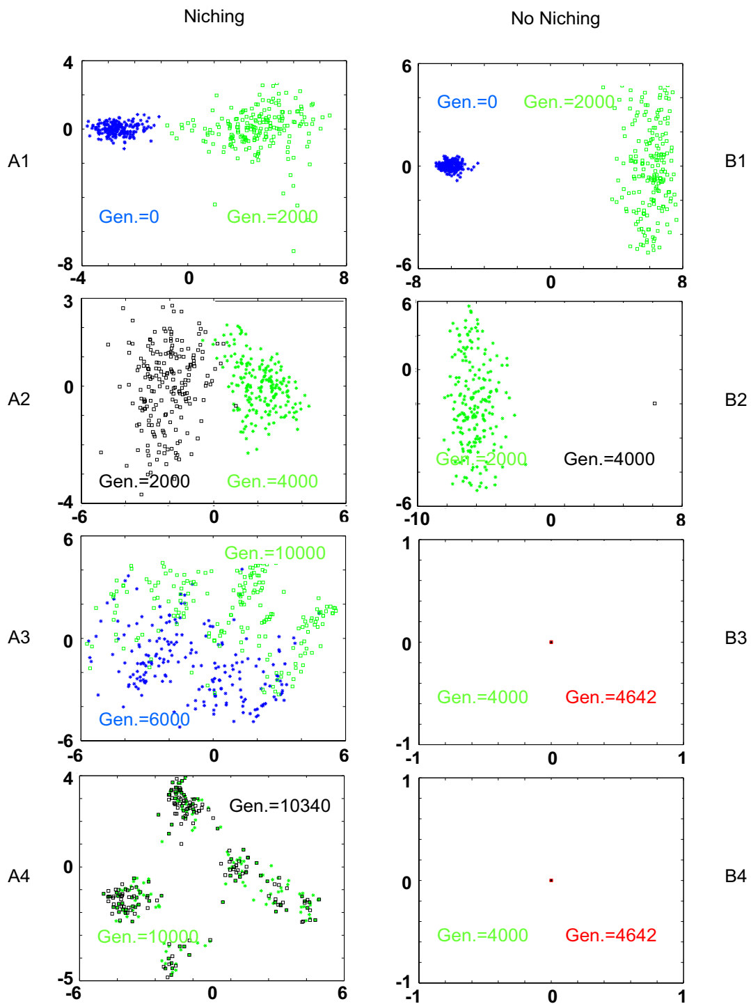
Figure 2 Evolution of the EA for a genetic algorithm with parental-recombination. These figures show the evolution of the distribution of the population during the learning process using parental-recombination with niching (A1-A4) and without niching (B1-B4). The populations were recorded every 2000 generations and after the algorithm's convergence. Each plot represents the graphs of two populations sampled consecutively. The graphs of both populations are represented as points on a 2D map using Kernel Principal Component Analysis .
