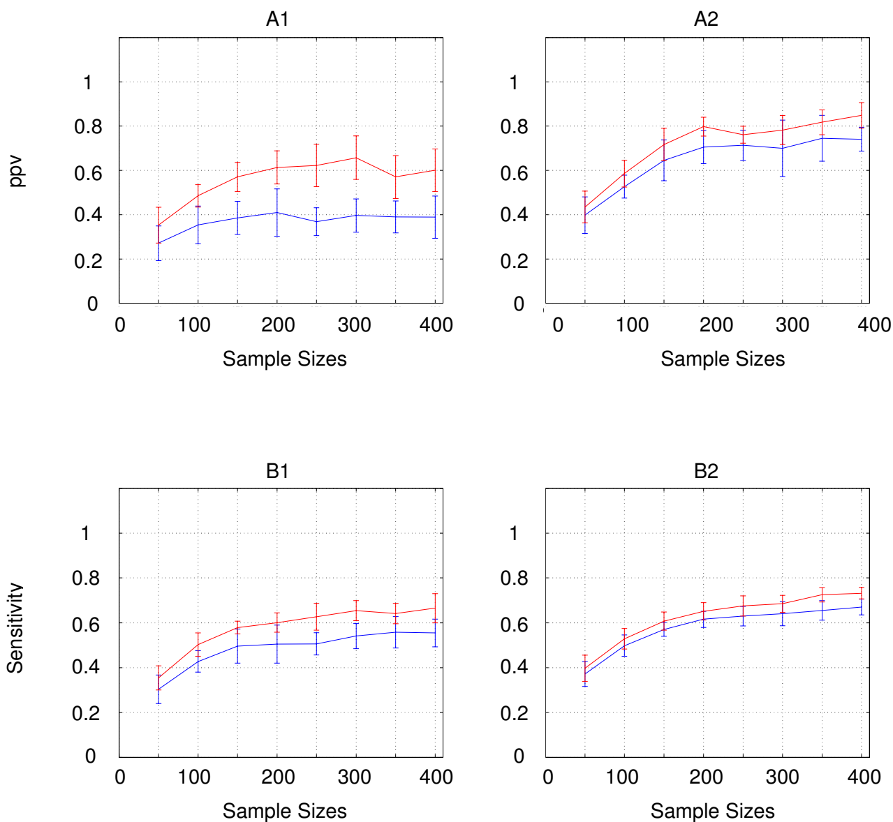
Figure 3 Comparison of the learning curves of parental-recombination and link-recombination. For each learning algorithm, the results of the comparison of the graph learnt for various sample sizes and the reference graph are expressed in terms of positive predictive value (A1 and A2) and sensitivity (B1 and B2). Figures A1 and B1 show the results obtained without niching, while Figures A2 and B2 show the results obtained with niching. The color coding is blue for parental-recombination and red for link-recombination. For each sample size, tests are performed on 10 different and independent datasets. The same datasets are used for every EA. Each point along the curves, which correspond to a given sample size, represents the mean value and the standard deviation of the quality measurement across the 10 runs of the algorithms.
