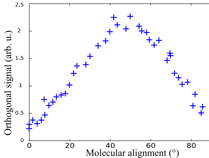
Figure 5. Evolution of the harmonic 21 orthogonal signal ( \varphi = 90^\circ ) as a function of the molecular alignment angle \theta .
