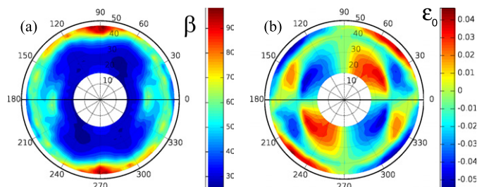
Figure 4. Polar plots of the measured decay rate \beta (a) and maximizing ellipticity \epsilon_0 (b) in \text{CO}_2 .
