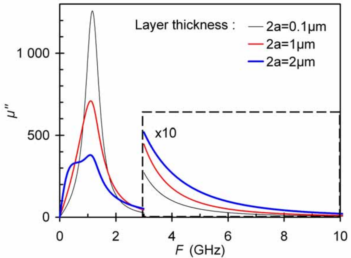
FIG. 2 The imaginary part of the permeability \mu'' computed for films with a thickness 2a ranging from 0.1\ \mu\text{m} to 2\ \mu\text{m} , using the Landau-Lifschitz-Gilbert model and taking into account skin effect.
