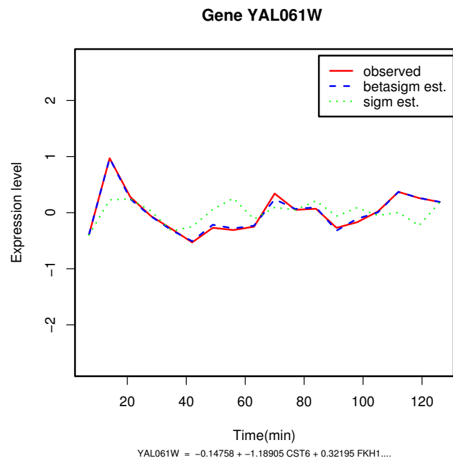
Figure 2 Comparative plot between the observed and the predicted values of mRNA expression levels of gene YAL061W. Example of good estimation of the expression profile with the beta sigmoid pattern of regulation: gene YAL061W.
